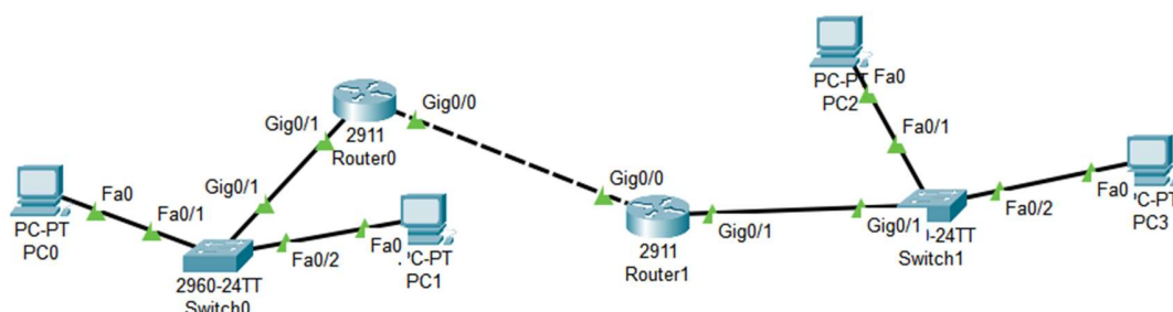
Figure 6.4: Topology of established network for OSPF routing protocol.
