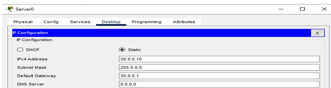
Figure 8.6: IP address, subnet mask and default gateway configured on Server0
