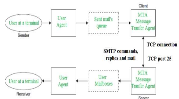
Figure 4.2: SMTP Model
