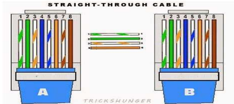
Figure 1.3: Straight-Through Cable Order Diagram
