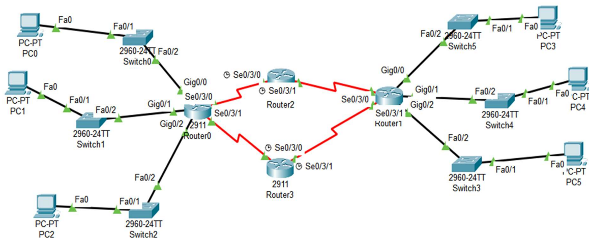
Figure 7.1: Topology of established network.
