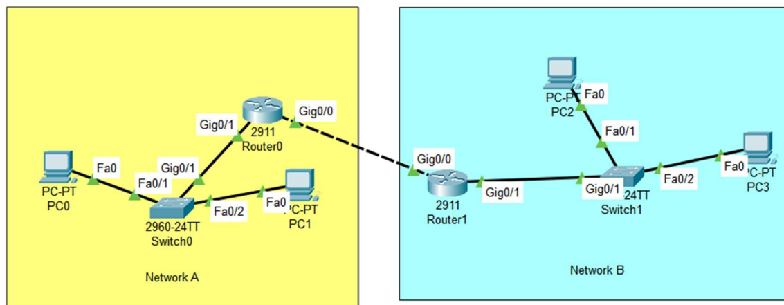
Figure 6.2: Topology of established network for static routing protocol.
