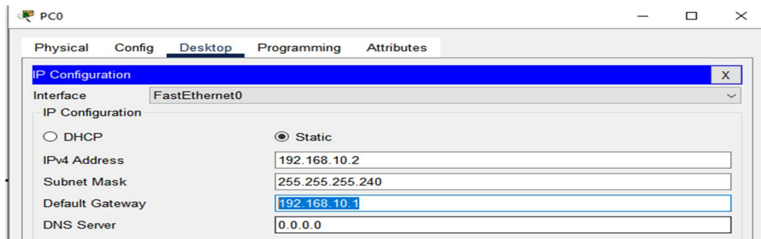
Figure 5.3: IP address, subnet mask and default gateway configured on PC0
