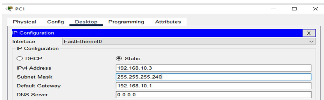
Figure 5.4: IP address, subnet mask and default gateway configured on PC1
