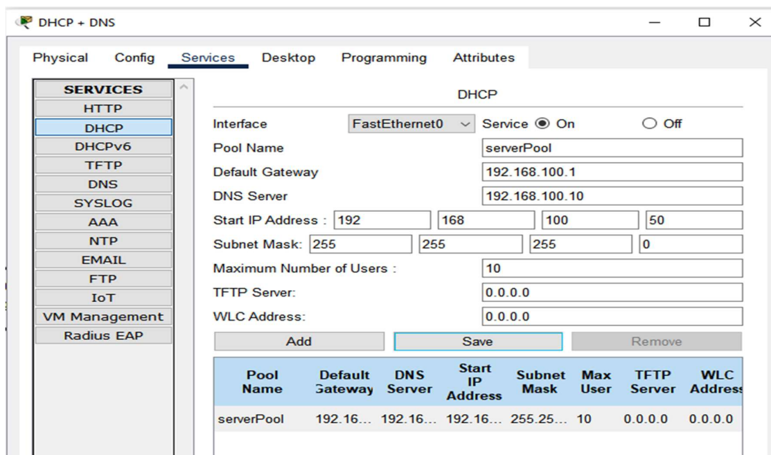
Figure 4.6: DHCP server configuration.
