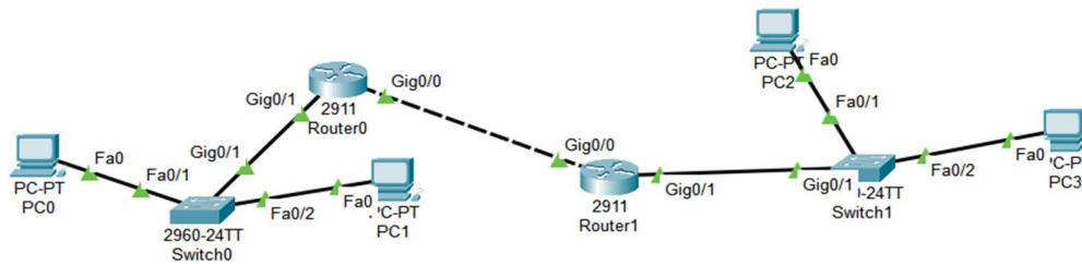
Figure 6.8: Topology of established network for RIP routing protocol.
