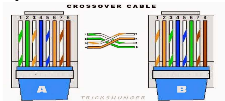
Figure 1.4: Crossover Cable Order Diagram
