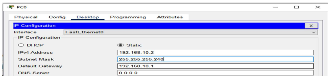
Figure 7.2: IP address, subnet mask and default gateway configured on PC0.
