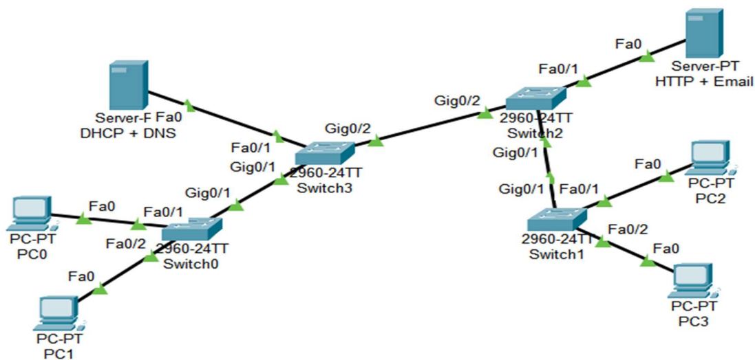
Figure 4.3: Topology of established network.
