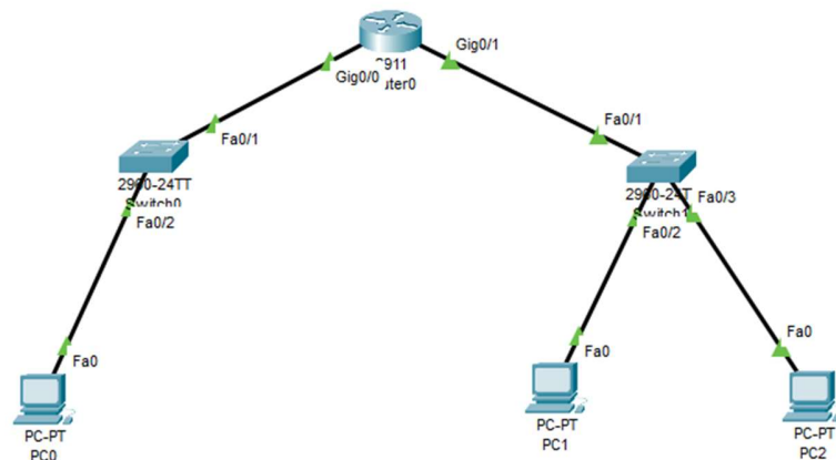
Figure 11.1: Topology of established network.
